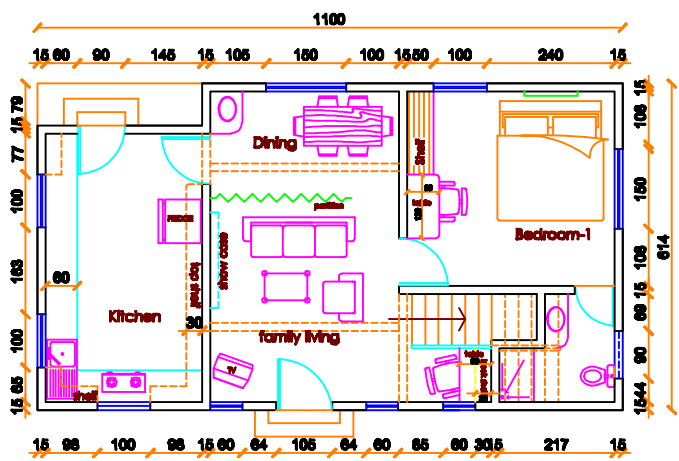
GROUND FLOOR AREA: 725 SQ.FT SCALE - 1:75
