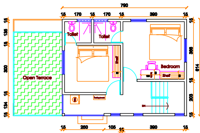
FIRST FLOOR AREA: 522 SQ.FT
