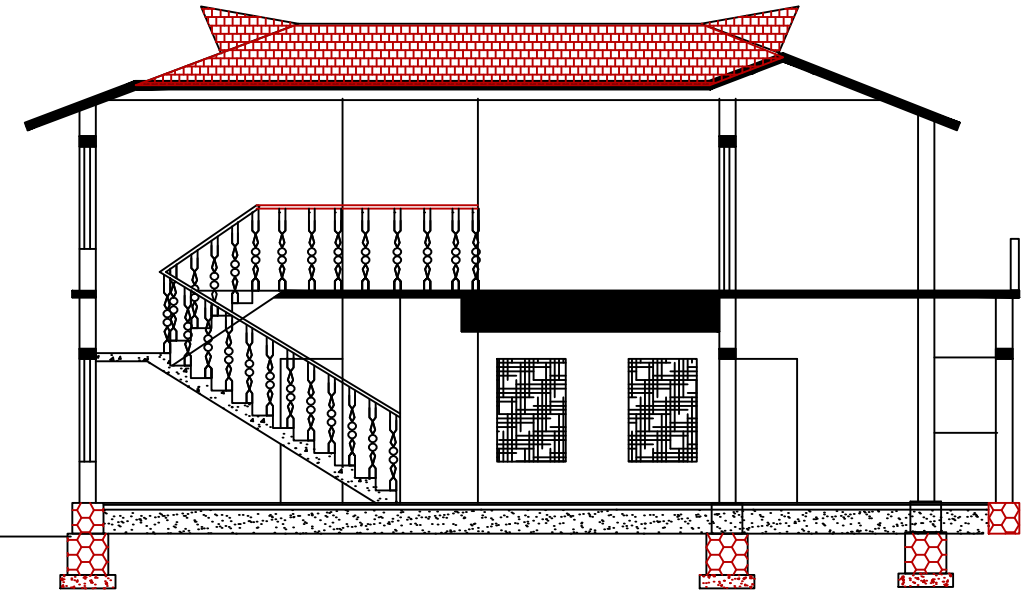
SECTIONAL ELEVATION AB
